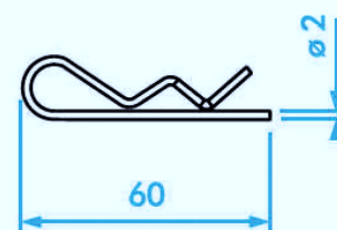
WKC Coppiglia Safety R-spring
