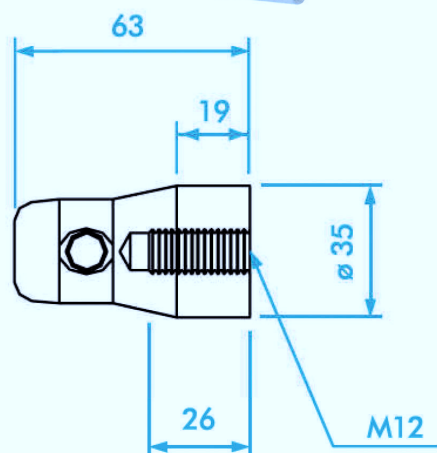
WKC Mezzo Spinotto allungato Offset half conical coupler
