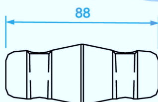
WKC Spinotto alluminio Conical coupler
